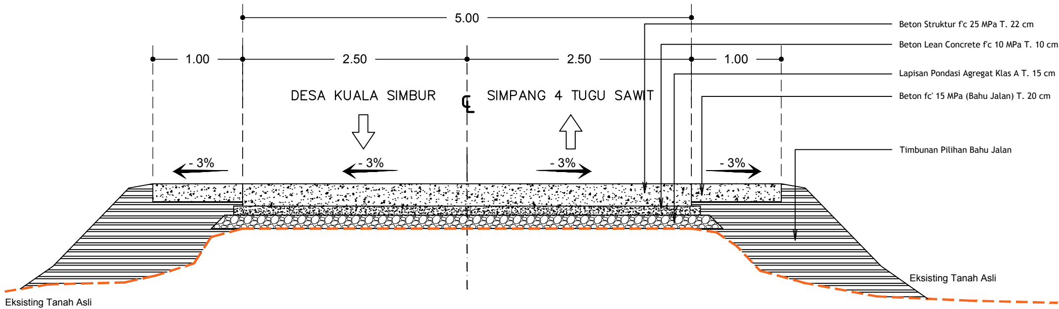
TYPICAL CROSS RENCANA Skala 1 : 100
