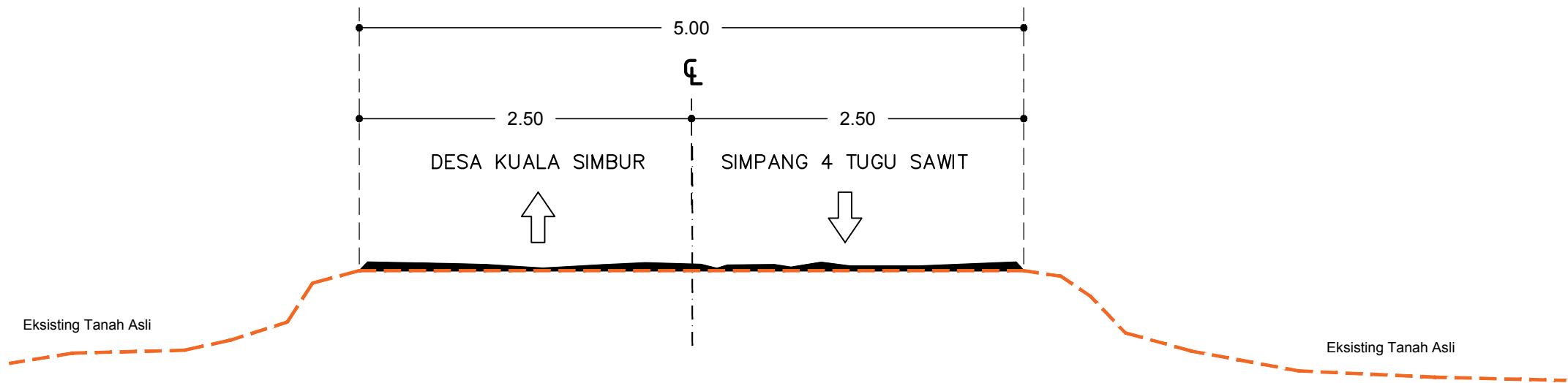
TYPICAL CROSS EKSISTING Skala 1 : 100
